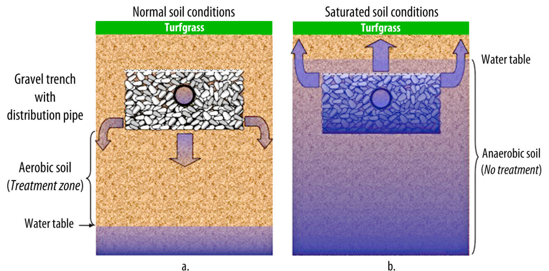
Figure 2. A cross section of an individual septic system soil treatment area trench.
